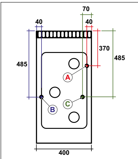
Fig. 11 Tank 400x700
