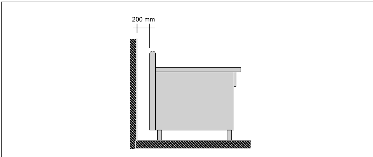
Fig. 13 Minimum distance from flammable walls
