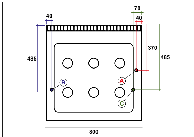
Fig. 12 Tank 800x700
