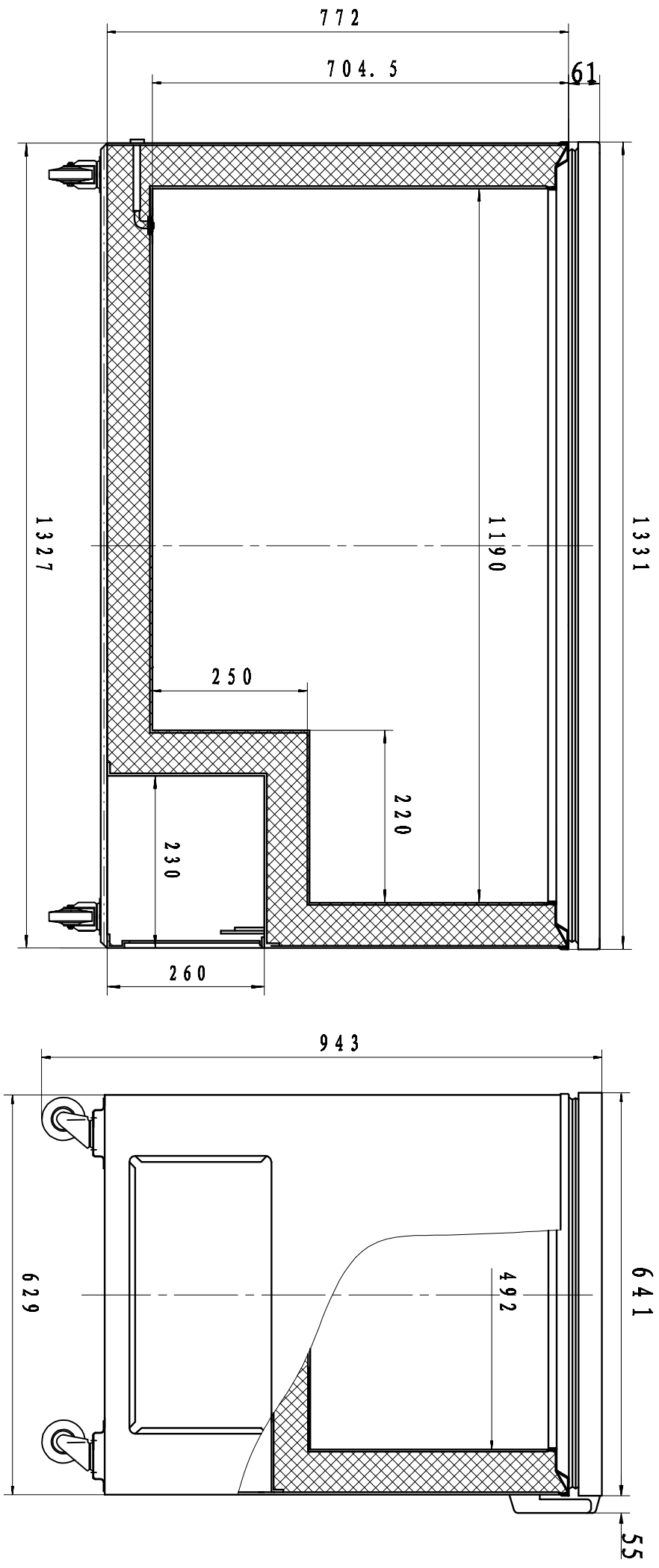
OUTSIDE DRAWING OF BD390
